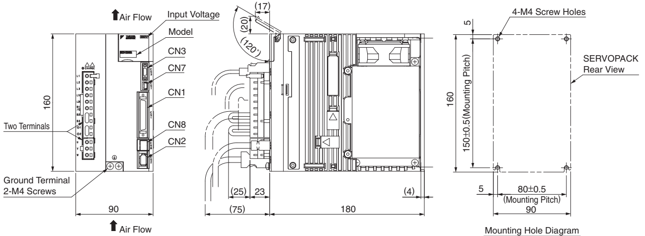
(6) Three-phase 200 VAC, Model: SGDV-120A0□A
