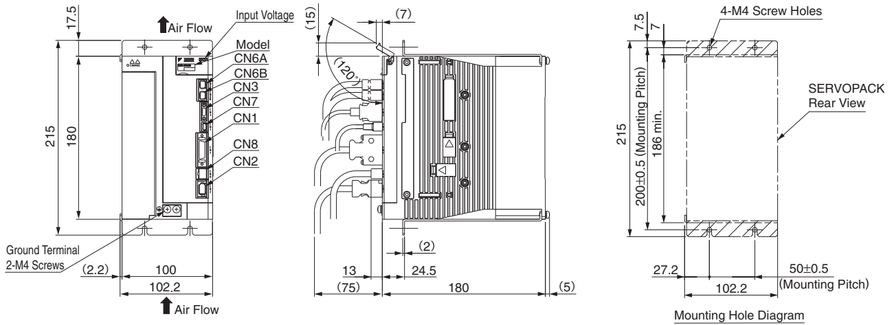
(8) Three-phase 200 VAC, Model: SGDV-330A2□A001
