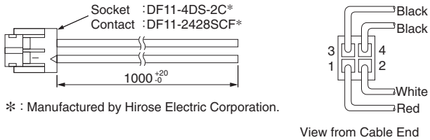
View from Cable End
