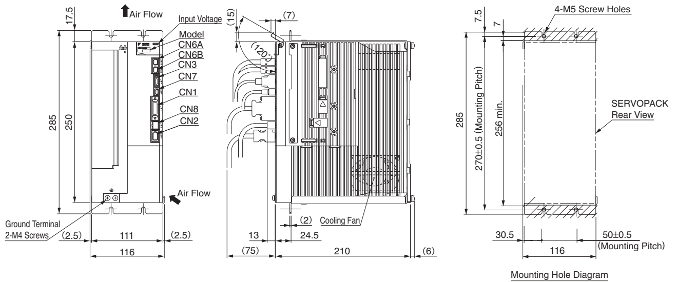
(8) Three-phase 200 VAC, Model: SGDV-330A2□A001
