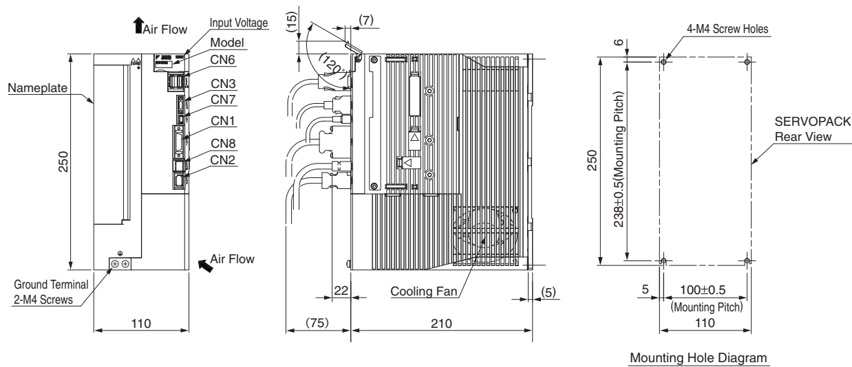
Mounting Hole Diagram Approx. Mass: 4.6 kg
