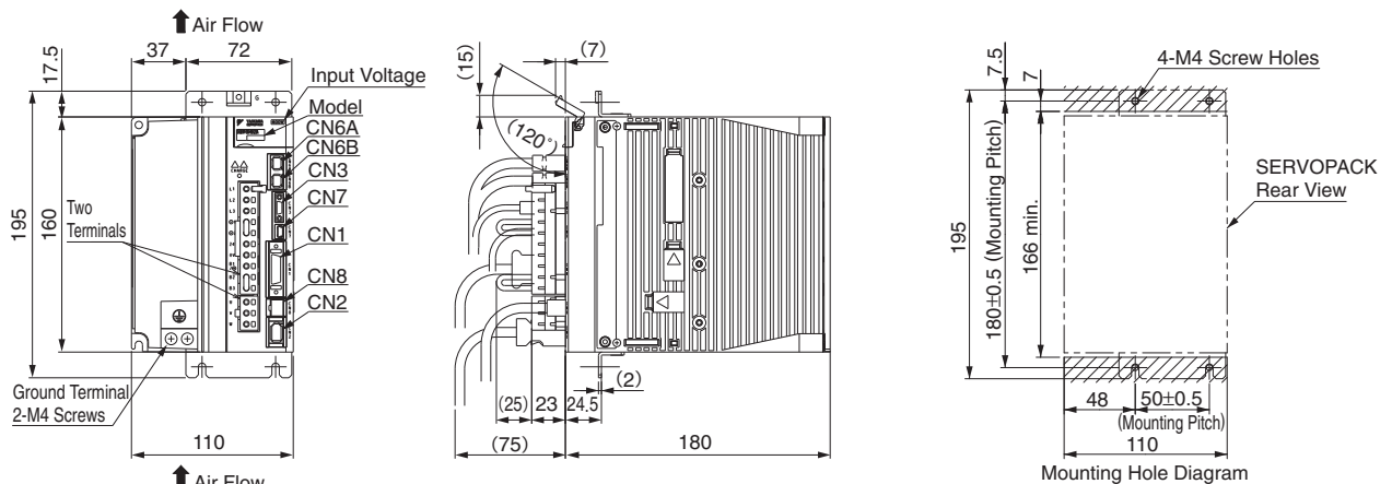
(9) Three-phase 400 VAC, Model: SGDV-1R9D2□A001, -3R5D2□A001, and -5R4D2□A001
