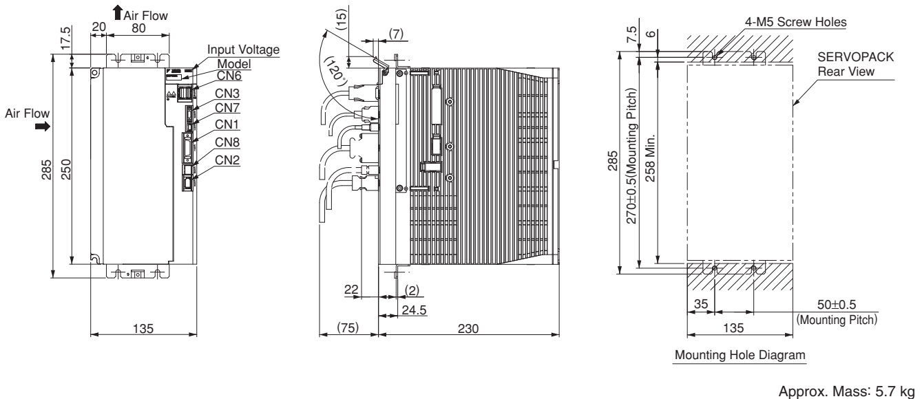
(13) Three-phase 400 VAC, Model: SGD1-170D1□A001
