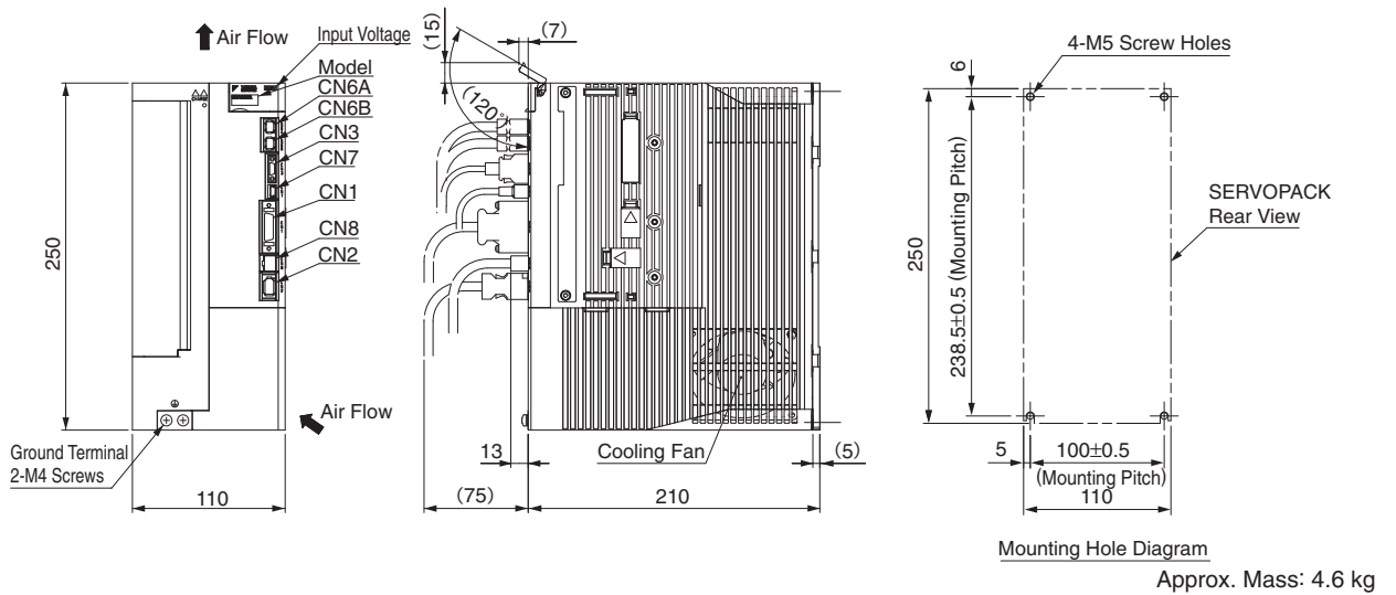
(8) Three-phase 200 VAC, Model: SGDV-330A2□A
