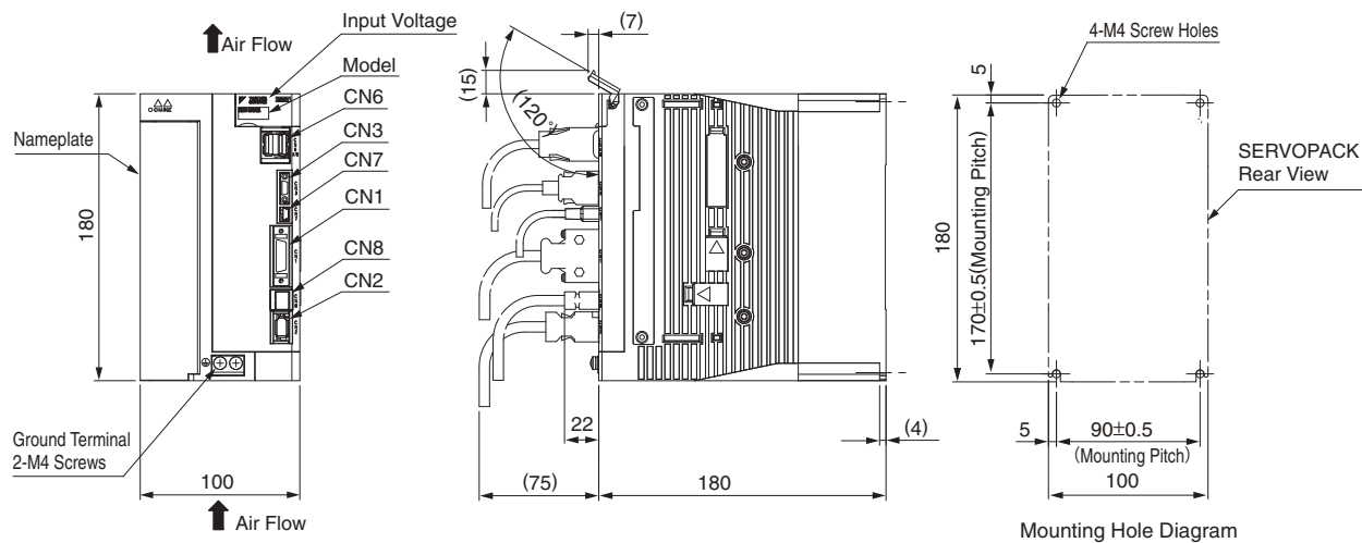
Mounting Hole Diagram Approx. Mass: 2.8 kg
