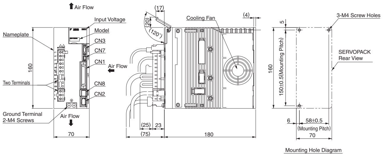
(5) Three-phase 200 VAC, Model: SGDV-3R8A0□A, -5R5A0□A, and 7R6A0□A
