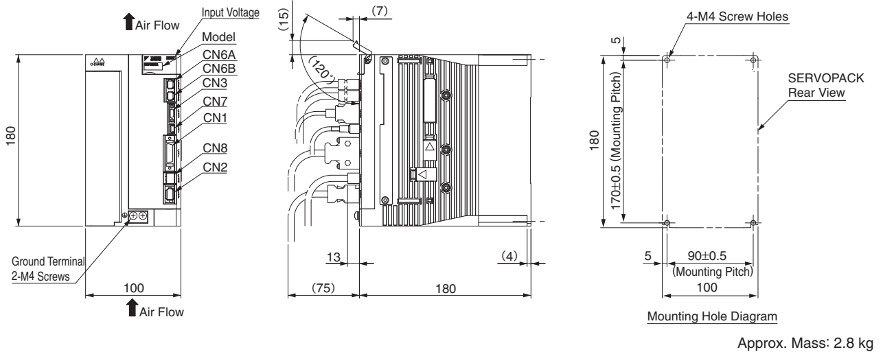
(8) Three-phase 200 VAC, Model: SGDV-330A2□A
