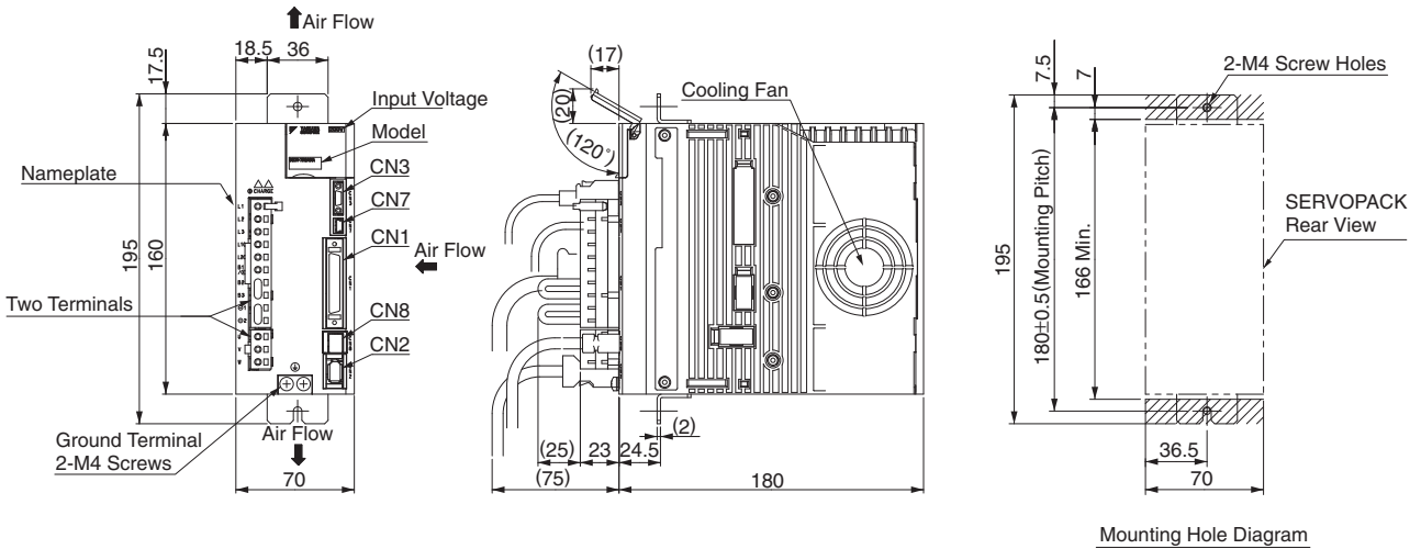
(5) Three-phase 200 VAC, Model: SGDV-3R8A0□A001, -5R5A0□A001, and -7R6A0□A001
