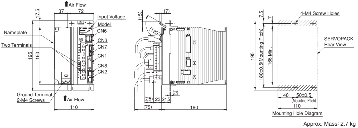
(12) Three-phase 400 VAC, Model: SGD1-8R4D1□A001 and -120D1□A001
