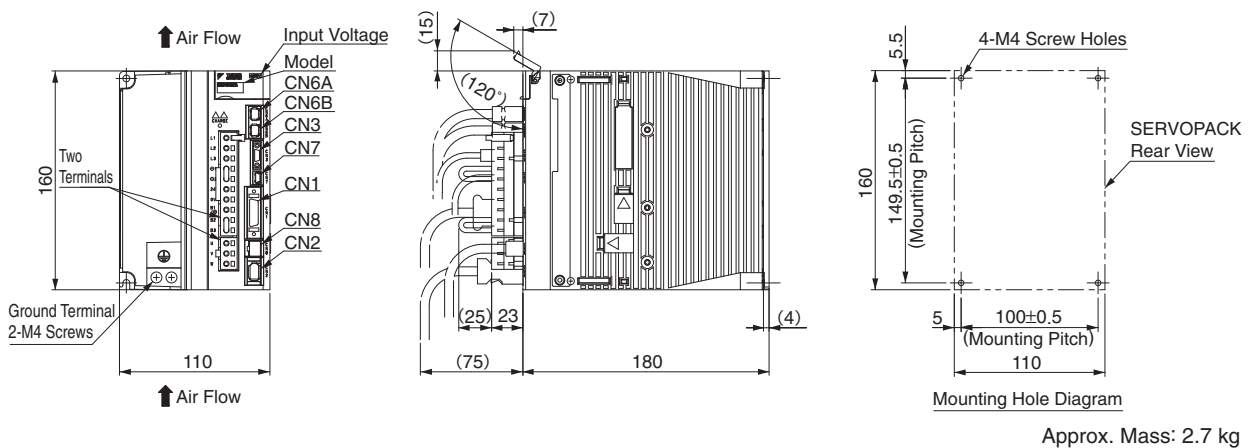
(9) Three-phase 400 VAC, Model: SGDV-1R9D2□A, -3R5D2□A, and -5R4D2□A
