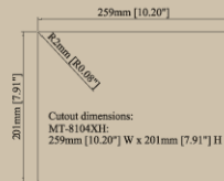
Panel Cutout
