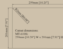
Panel Cutout
